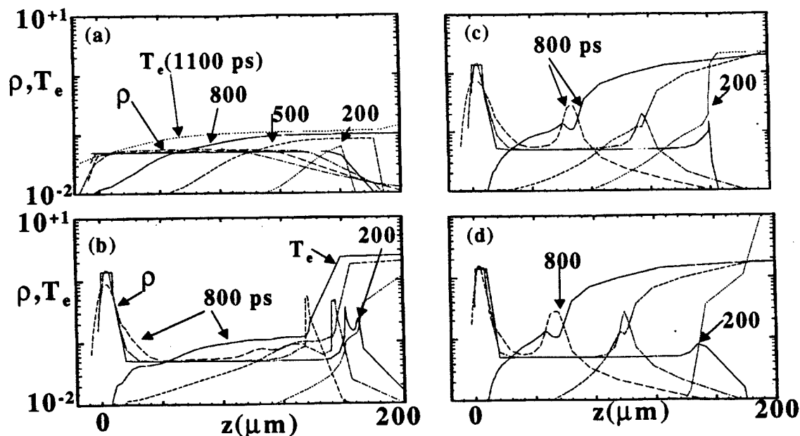
Figure 2. Evolving electron temperature T_e (keV) and plasma density \rho ( \text{gm}/\text{cm}^3 ) under the Fig. 1 (b) pulse for: a) a 1500 Å gold layer displaced 3000 Å to the right of the foam, (b) the same gold layer directly attached to the foam and with a CH layer added behind the foam, (c) with the gold layer reduced to just 250 Å, and (d) with the gold layer replaced by 1 μm of CH. Progressively, stronger shocks are seen as the gold layer is first attached and then thinned.
